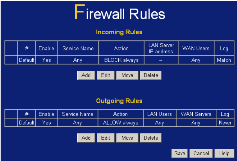
Figure 29 Firewall Screen
